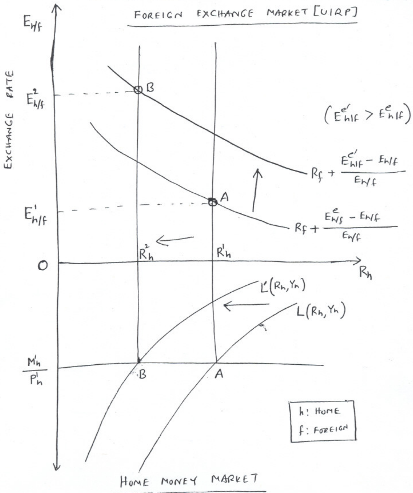
FIGURE 1: SHORT-RUN EFFECTS
