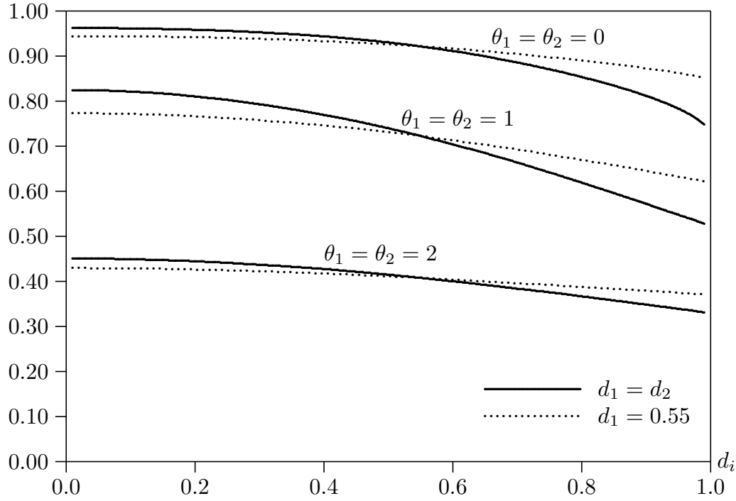
Figure 4. Dependence of rejection frequencies on canonical correlations
