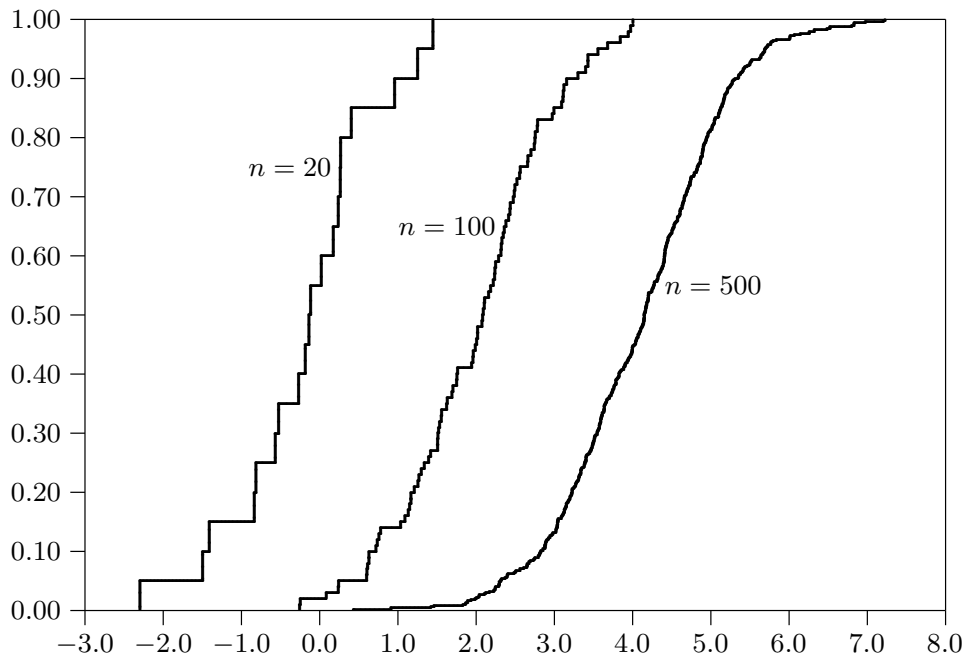
Figure 4.6 EDFs for several sample sizes
