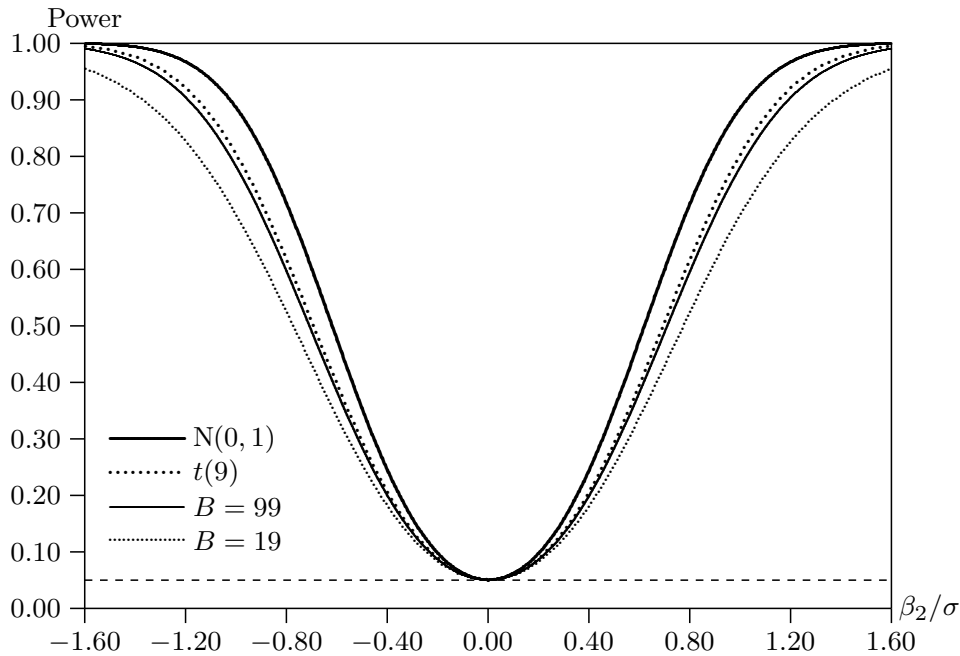
Figure 4.11 Power functions for tests at the .05 level
