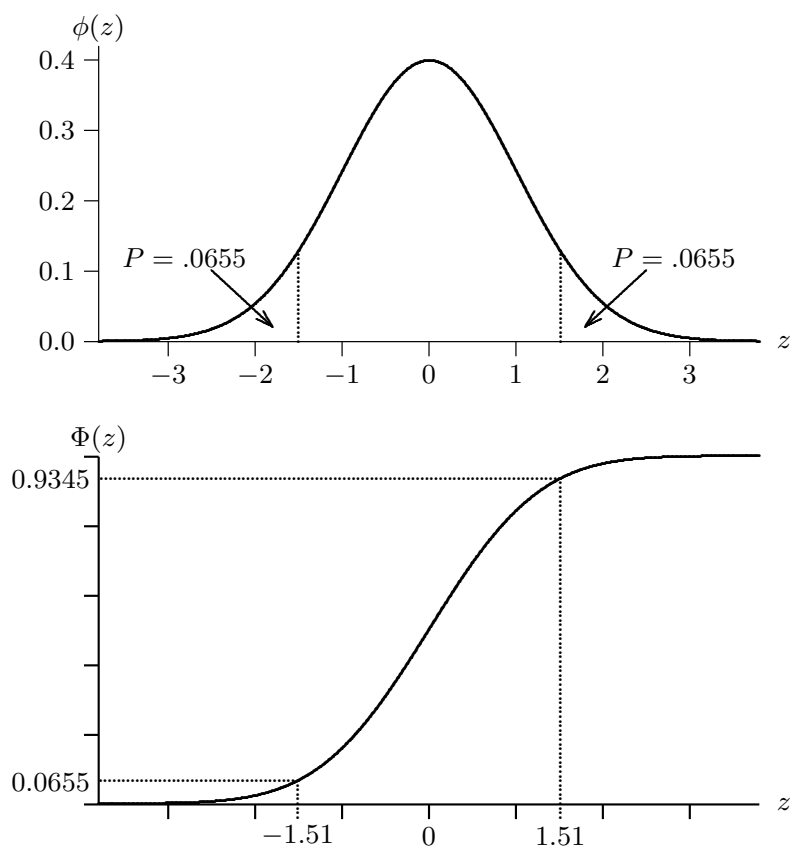
Figure 4.2 P values for a two-tailed test
