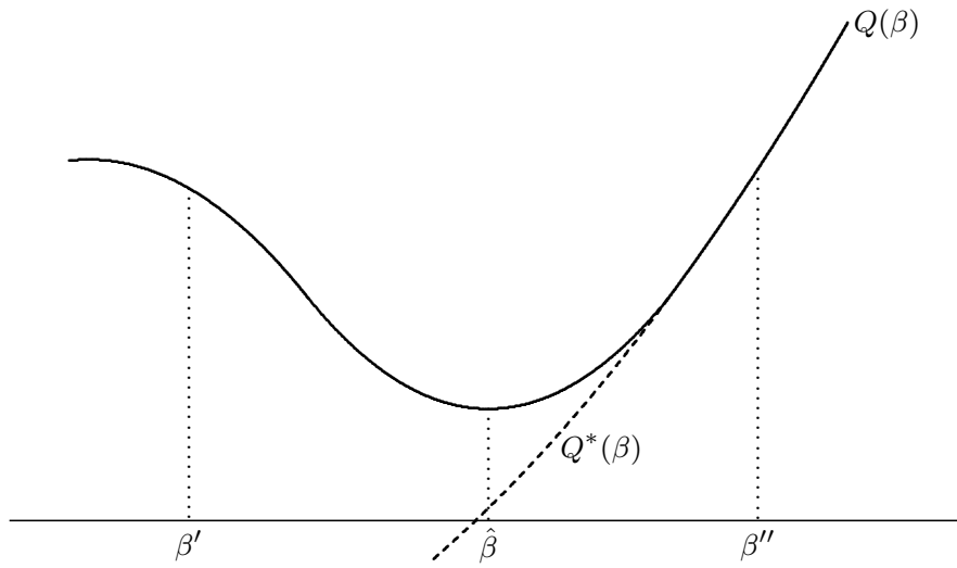
Figure 6.2 Cases for which Newton's Method will not work
