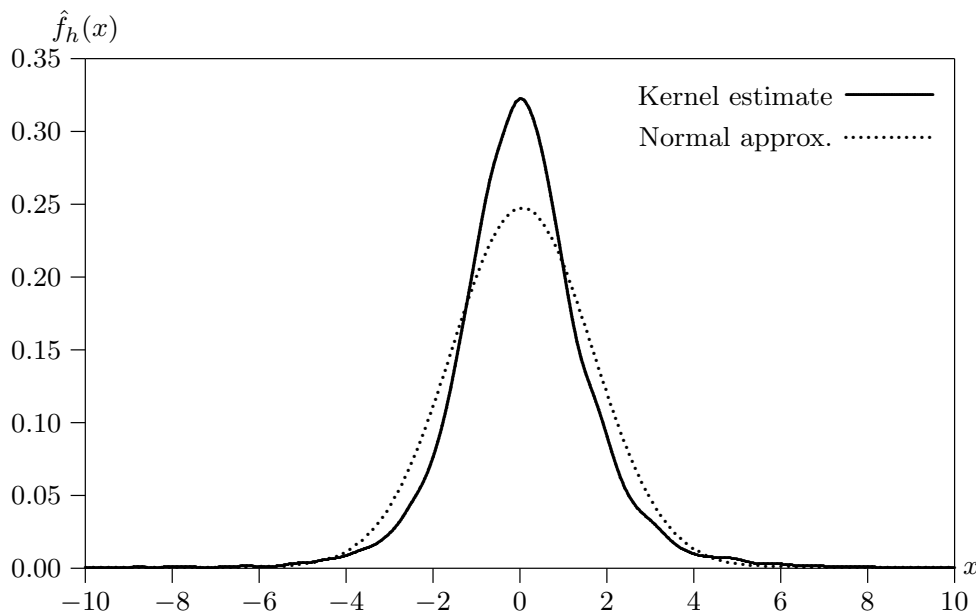
Figure 15.1 Estimates of the density of IBM stock returns
