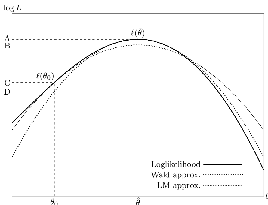
Figure 10.3 LR, LM, and Wald Tests
