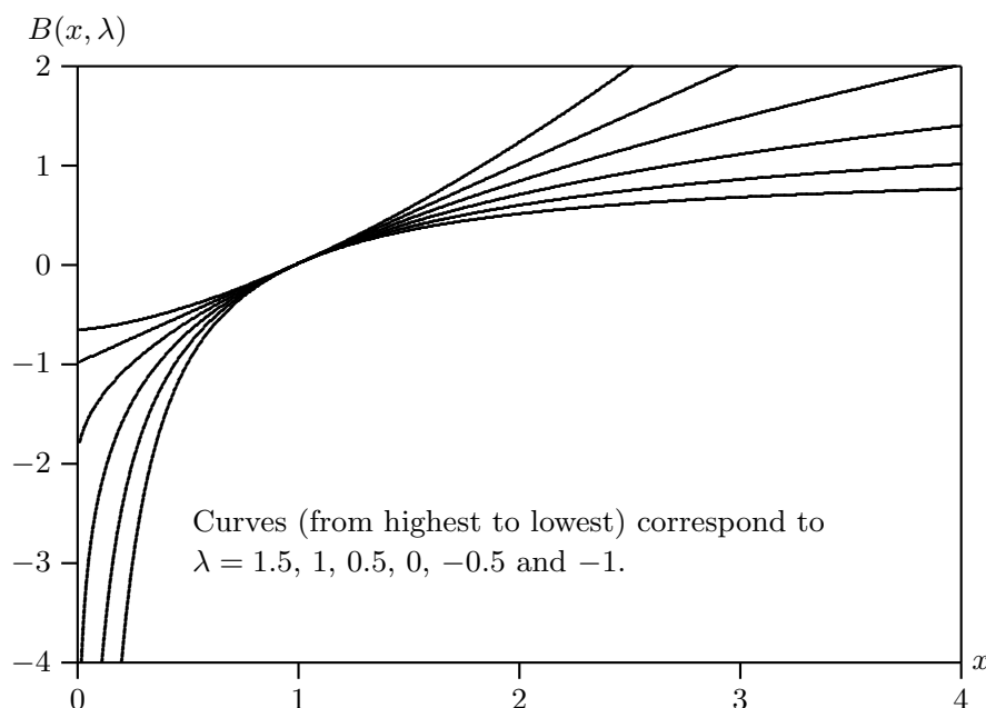
Figure 10.4 Box-Cox transformations for various values of \lambda
