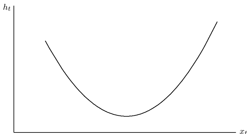
Figure 2.15 A graph of h_t as a function of x_t
