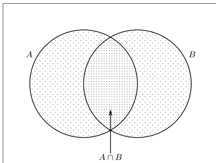
Figure 1.3 Conditional probability
