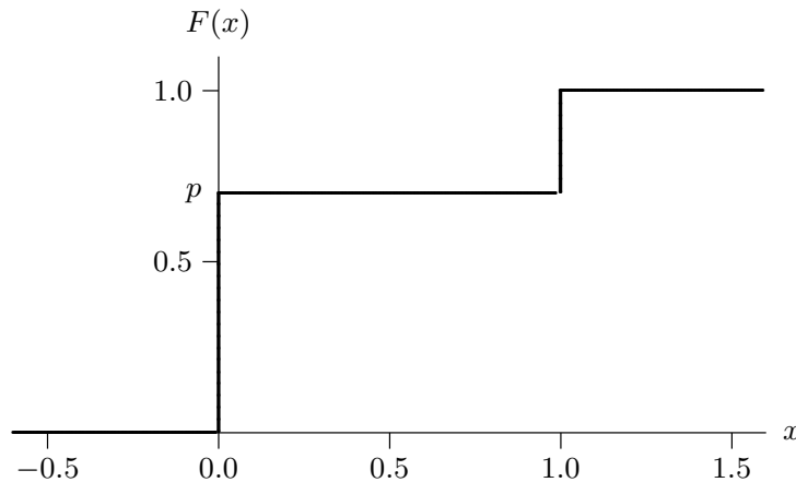
Figure 1.2 The CDF of a binary random variable
