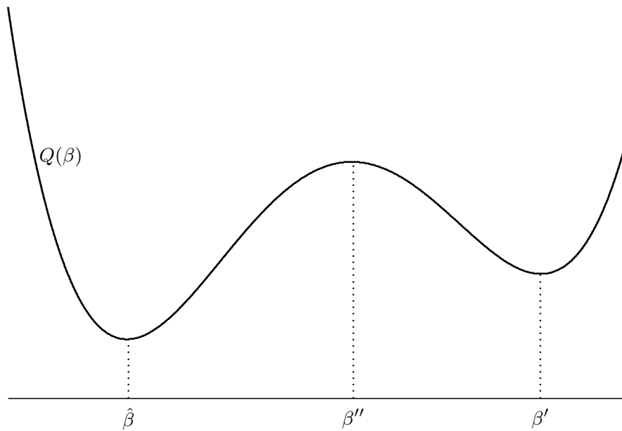
Figure 6.3 A criterion function with multiple minima
