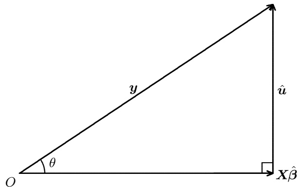
Figure 2.10 Residuals and fitted values
