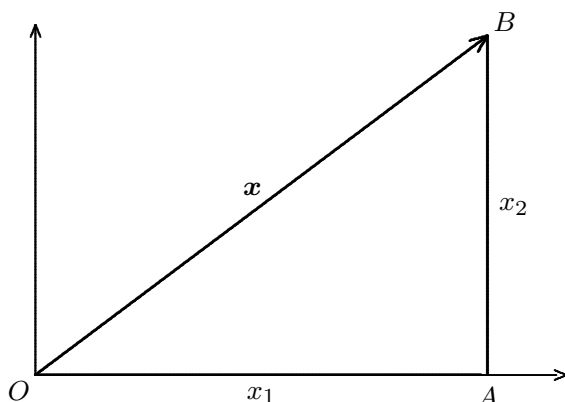
Figure 2.3 A vector \mathbf{x} in E^2
