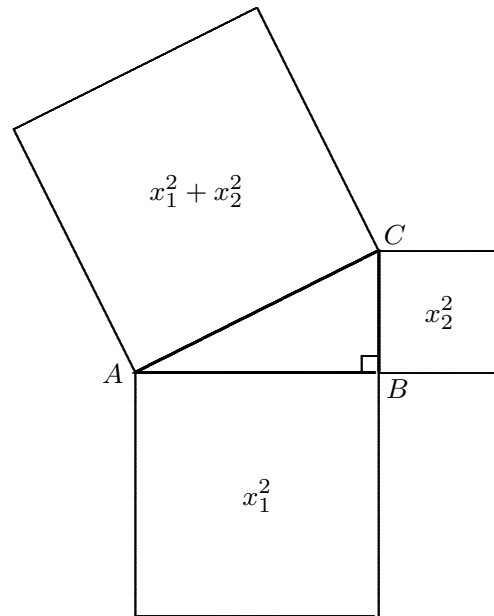
Figure 2.1 Pythagoras' Theorem
