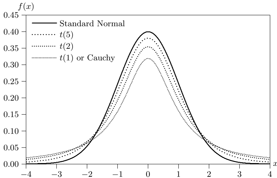
Figure 4.5 PDFs of the Student's t distribution
