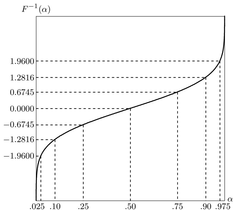
Figure 5.1 The quantile function of the standard normal distribution
