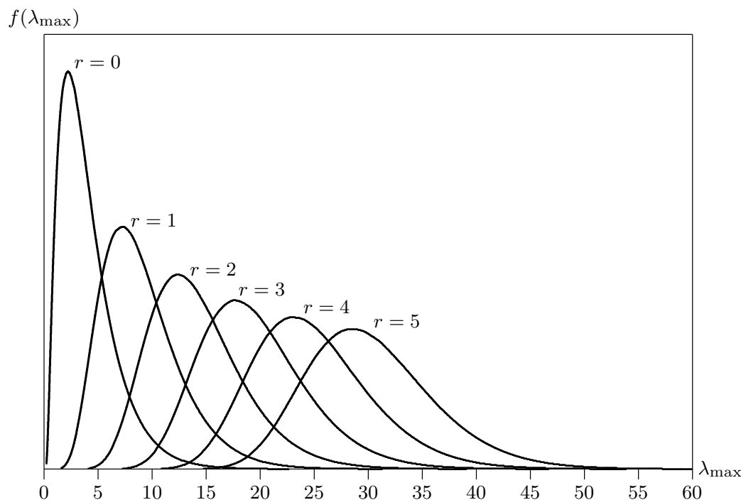
Figure 14.6 Asymptotic densities of some \lambda_{\max} tests
