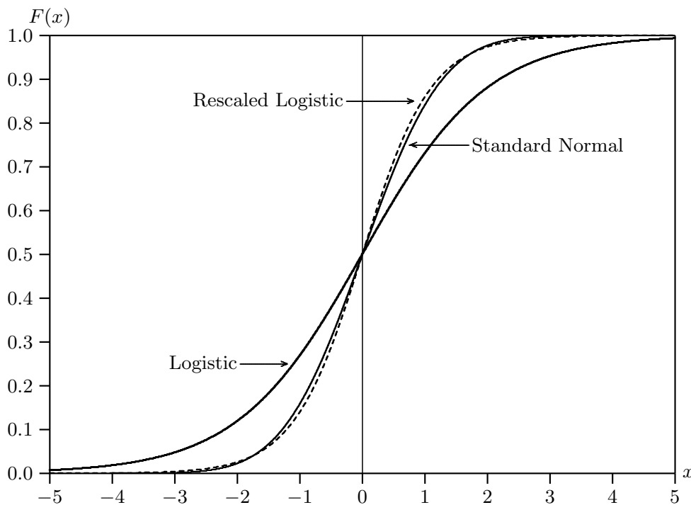
Figure 11.1 Alternative choices for F(x)
